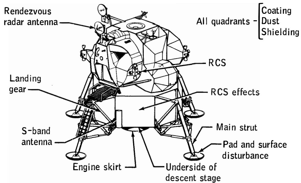
Figure 3-5. - Quad I inspection points.
