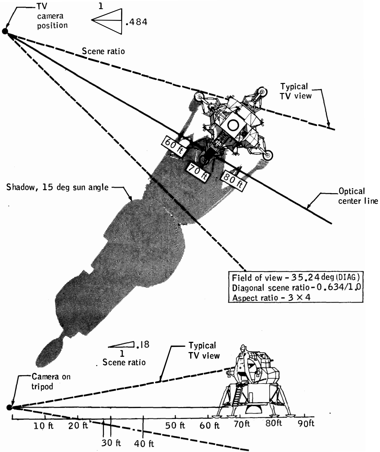
Figure 3-4.- TV field of view from tripod (with Lunar day lens)
